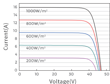
Current-Voltage Curve JAM66D45-600/LB
