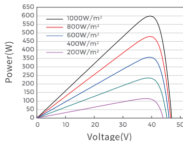
Power-Voltage Curve JAM66D45-600/LB
